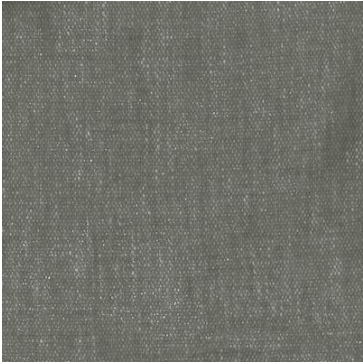
Shale
